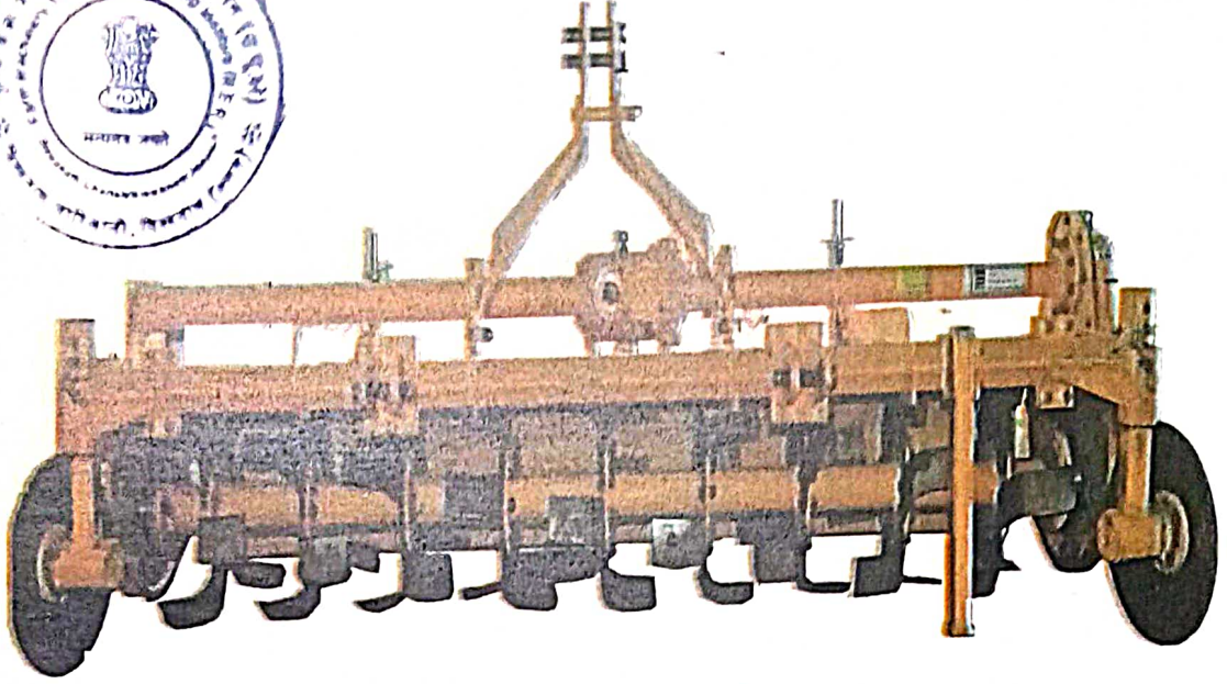
SWAN AGRO ROTARY TILLER (ROTAVATOR), MODEL: NSML RTJT 225 MULTI SPEED, GEAR DRIVE, CENTRALLY MOUNTED
