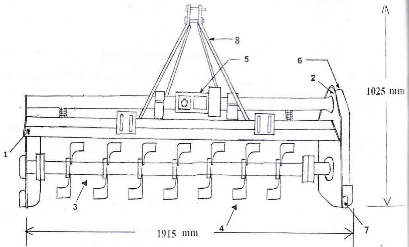
Fig.1: NEW SWAN (NSE RT 150) SS Rotavator
