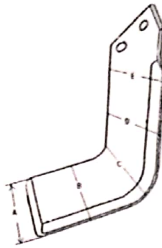
Fig 7 : DIMENSIONS FOR WEAR ANALYSIS
