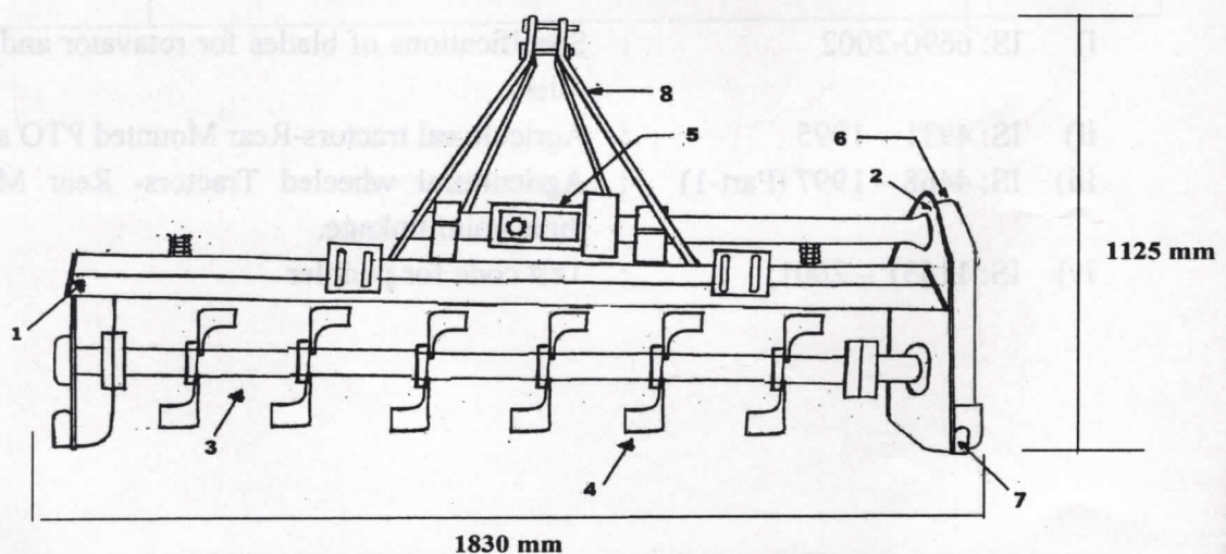
Fig.1: SHAKTIMAN (SRT 5.5/MS Light Series) Rotavator
