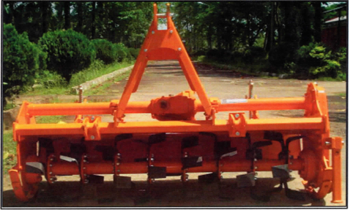
SHAKTIMAN (SRT 5.5/MS Light Series) Rotavator
