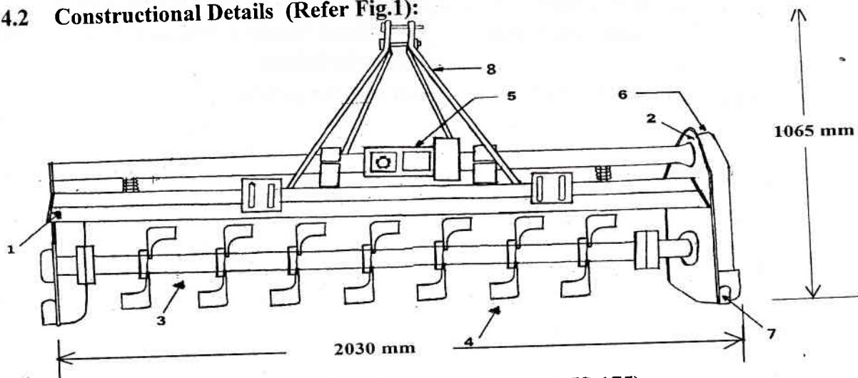
Fig.1: Baba Rotavator (BRTG MS 175)
